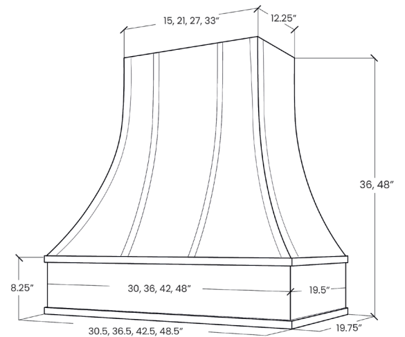
Curved with Strapping & Flat Trim
