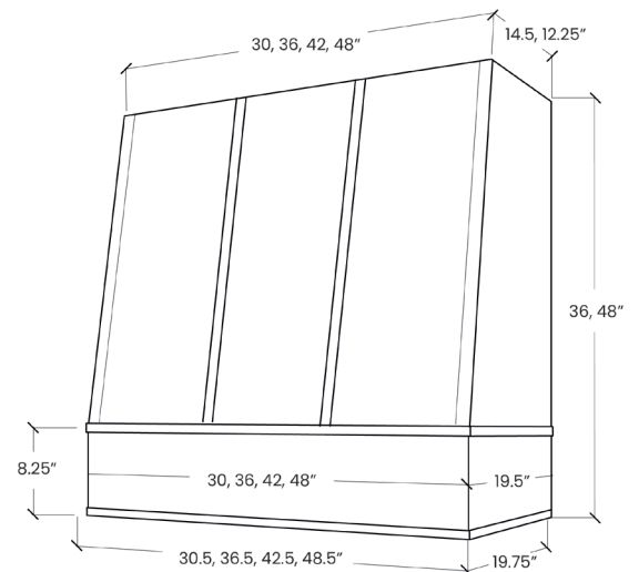
Angled with Strapping and Flat Trim
