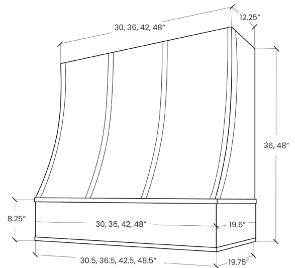
Sloped with Strapping & Flat Trim
