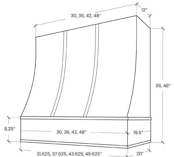
Sloped with Metal Strapping
