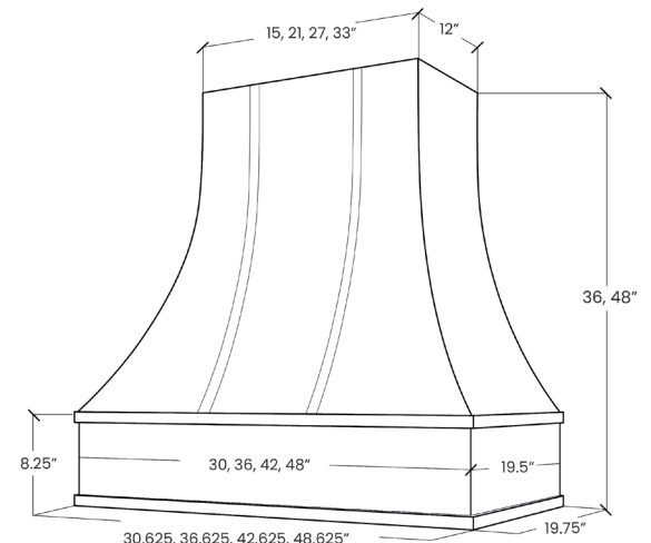
Curved with Metal Strapping
