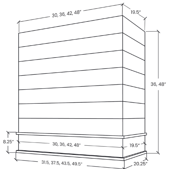
Box with Shiplap and Block Molding
