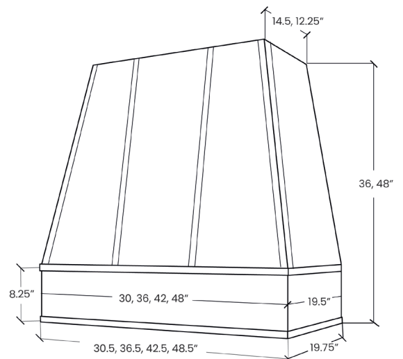
Tapered with Strapping and Flat Trim
