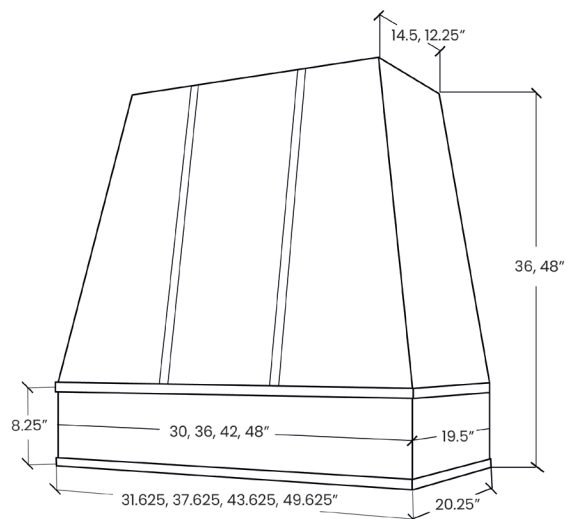
Tapered with Metal Strapping
