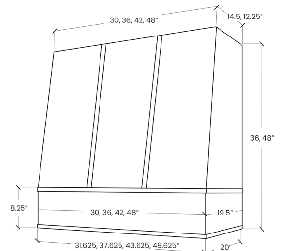
Angled with Metal Strapping
